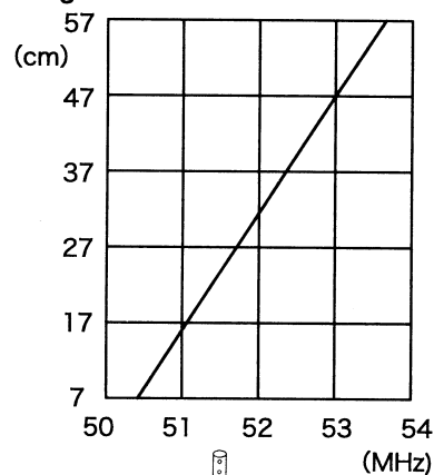
Frequency rage per Insertion length
