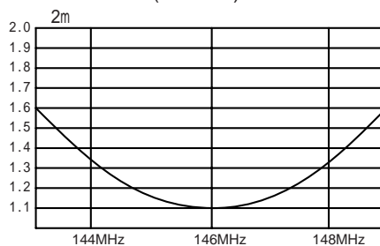
V.SWR chart (X-50NA)
