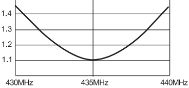
V.SWR chart (X-300N)
